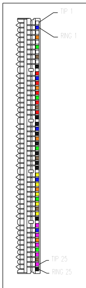
Figure 1- Incoming 710 Connector
